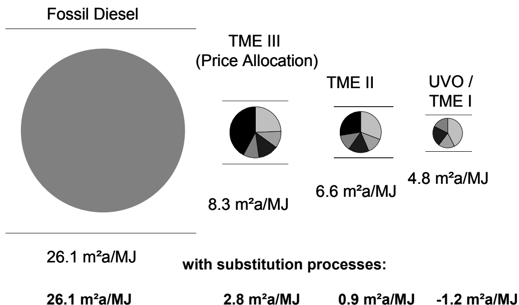
Figure 4-3: The Sustainable Process Index of different scenarios for Biodiesel compared to fossil Diesel
